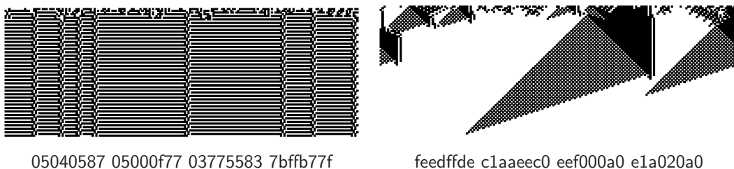
Figure 18.1: Transforming rcode: Left : the space-time patterns of a 1d density classification rule from[13] does not appear as intended because the order convention is the opposite of DDLab's. Right : after the rule is inverted to DDLab's convention the density rule behaves correctly. n=199 , v2k7 . The same random initial state is used in both cases. The rule-tables are shown in hexadecimal.
