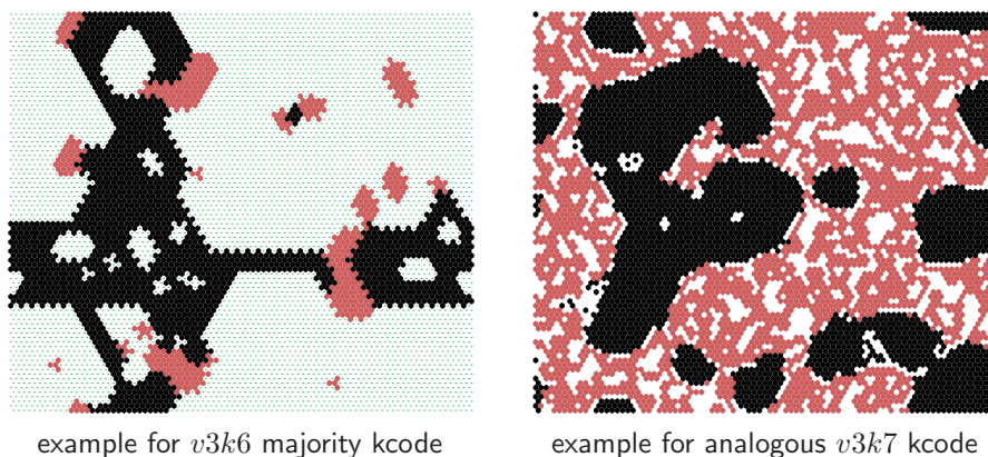
Figure 16.14: The effect of inserting a random string within a v3k6 kcode majority rule to create an analogous v3k7 kcode. The figures show space-time pattern snapshots from random initial states on a 88 \times 88 hexagonal lattice. Some aspects of the majority behavior are retained in k7 . Note that there are many possibilities for both examples — the actual kcodes are as shown in this section.
