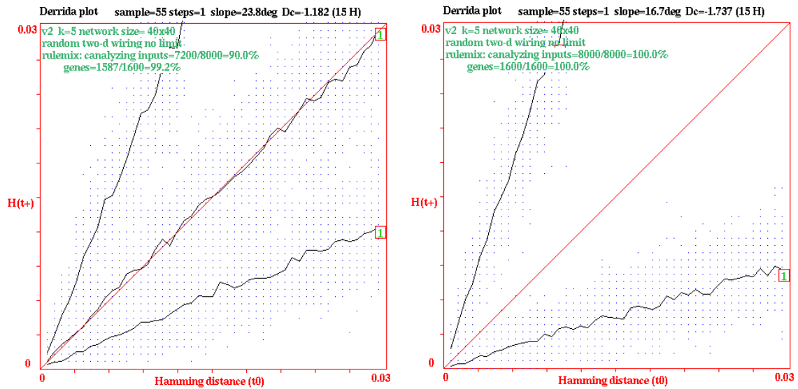
Figure 22.2: Examples of Derrida plots and their Derrida coefficients ( D_c ) for a 2d RBN, k=5 , n=40 \times 40 with various canalizing, settings C\% , changed in section 22.5 for a range of behavior. Other parameters were as follows: D_c sample=15, \text{MaxH}=0.03 , sample=55, iterations=1, steps=1. The average slope, \delta^\circ , and the Derrida coefficient, D_c , for the plots are given below.
