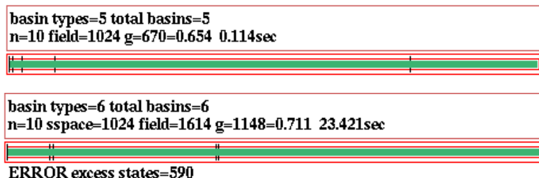
Figure 30.1: Examples of the basin of attraction field progress bar and the data window, for an RBN. Top: For a normal run without error. Bottom: An example where the wiring was changed during a pause, leading to inconsistent data where the size of the field is greater than state-space. The progress bar has gone off its scale on the right.
