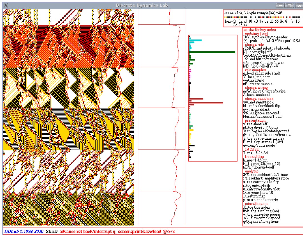
Figure 32.8: A snapshot of the DDLab screen, showing 1d n=200 space-time patterns, a series of “glider” rules from the v4k:3 complex rcode collection loaded on-the-fly with key g . The start of each new rule, which preserves the current state, is indicated by a horizontal line on the entropy plot to the right of the space-time pattern. The last rule set is shown in a top-right window, including its sample number.
