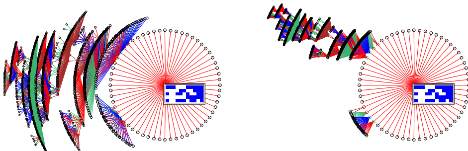
Figure 26.12: Decreasing the pre-image fan-angle of a subtree of a 1d CA v2k3 rcode(dec)110 , n=55 . The subtree root, (hex)71f0cf34c0fced, is highlighted as a bit pattern. Other nodes are show as spots. Left: default fan-angle (factor=1). Right: reduced fan-angle (factor=0.3). Note that the fan converging on the root of a subtree is always 360^\circ , and is not affected.
