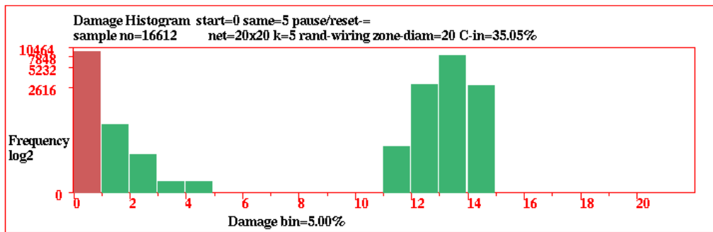
Figure 31.17: The damage histogram with the damage frequency allocated to 20 equal size bins, shown with the y axis in log form. This is a similar network as in figure 31.15, but with canalizing inputs set to 35%, resulting in less ordered dynamics and a bimodal distribution of damage frequency.
