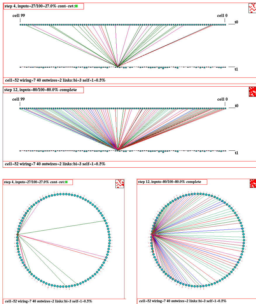
Figure 17.7: Recursive inputs (direct and indirect) to a given cell for a k=2, n=100 RBN. Above: As time-steps. Below: As a circle. Firstly, inputs are shown after 4 backward steps with 27 cells reached. Secondly, the complete inputs are shown after 12 backward steps with 80 cells reached. A small 2d insert in the top-right hand corner of the wiring window graphically indicates the fraction of cells connected so far.
