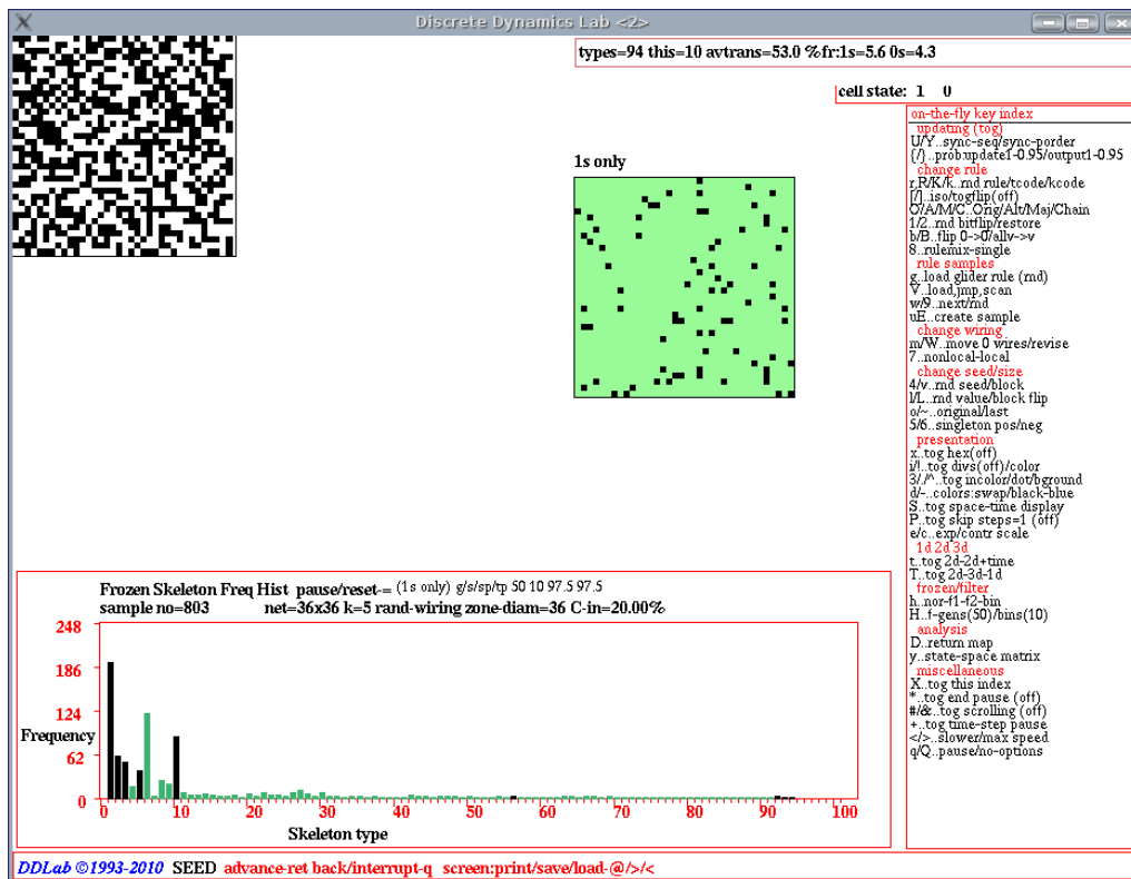
Figure 31.23: A snapshot of the DDLab screen, showing the skeleton histogram at sample 803 with 94 skeletons found.. The network is a 36 \times 36 v2k5 RBN with unbiased random wiring and 20% canalyzing inputs (chapter 15). The parameters in section 31.8 (1s only), labelled g/s/sp/tp , are 50, 10, 97.5%, 97.5%. Each sample starts with a new random initial state, and the skeleton into which the transient falls is identified (if any). A skeleton that cannot be matched with a pre-existing type is added as a new type. The histogram columns are continuously updated (in black), showing the skeleton type ( x axis) against the frequency of arriving at that type ( y axis). The axes rescale automatically (and columns turn green) on reaching the current scale limits. Top left: a snapshot of the space-time pattern. Top center: the skeleton, pattern of frozen 1s. Bottom: the unsorted histogram.
