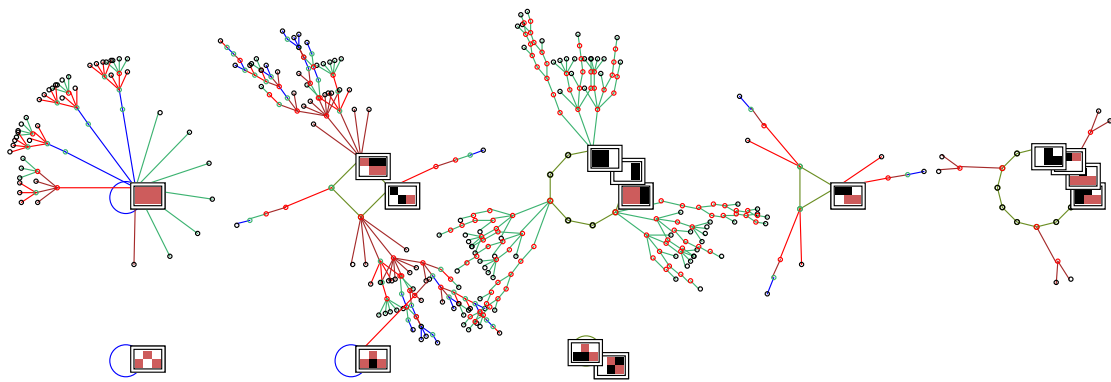
Figure 4.2: The basin of attraction field of multi-valued v3k3 n=6 1d CA. The lookup table is 120201201020211201022121111 (1886122584a655 in hex). Just the 8 nonequivalent basins are shown from a total of 23, and attractor non-equivalent states are shown as 2d patterns. State-space= v^n=3^6=729 . Note that the overlap can be fixed with layout options (chapter 25 or section 20.14).
