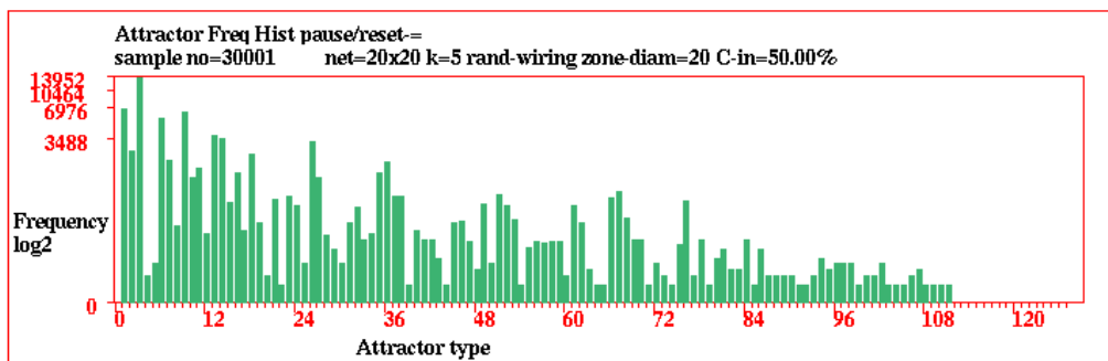
Figure 31.20: The attractor histogram for a sample of 30001 and 111 attractors, sorted by attractor period and average transient length, with log y -axis. (section 31.7.4).
