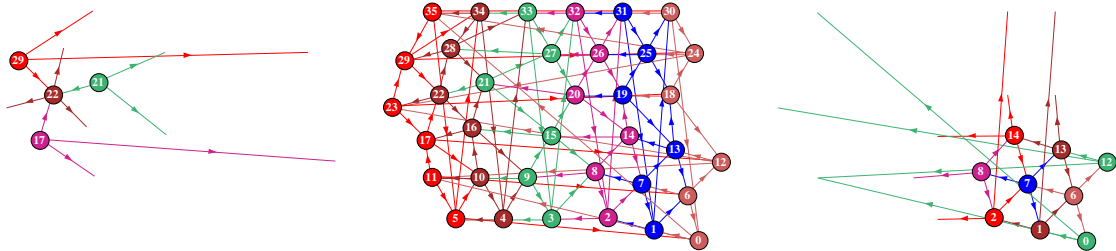
Figure 20.11: Isolating fragments in a 6x6 2d network-graph with a k=3 triangular n -template (section 10.1.2.) Center : The graph with a linked fragment and a block both slightly dragged and rotated. Left : The isolated linked fragment centered on node 22 according to “inputs” and “step=1”. Right : The isolated “block” defined between nodes 14 and 0.
