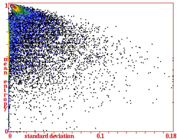
Figure 33.12: The rule sample scatter plot, showing a 1d rcode sample with 17680 unbiased random rules (file v2k5ss.sta ), sorted by standard deviation entropy. A color scheme indicates frequency. To select a rule anywhere on the plot, click on a point with the left mouse button for a list, then select the rule (sections 33.9, 33.5).
