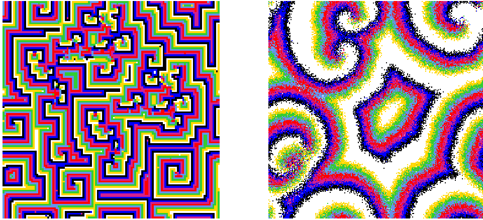
Figure 13.5: Reaction-Diffusion dynamics, 2d. Left: v8k8 , threshold interval is 1 to 6, 122x122 square lattice. Right: v8k11 , threshold interval is 2 to 7, 255x255 square lattice, random connections within a 24 diameter local zone.
