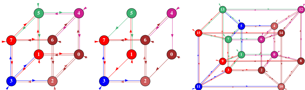
Figure 12.1: Hypercube wiring shown as a network-graph (section 20.5). Left: n=8 k=4 hypercube, which includes self-links. Center: a degraded version of the n=8 hypercube with some links missing. Right: n=16 k=5 hypercube. The 3d-3 network-graph option was used for the figures, and the graph was rearranged by dragging nodes (section 20.10). The figures should be viewed as if looking up from below. Output directed links are the same color as the source node. To regenerate these layouts automatically, enter file-f in section 20.7.3 for the filing prompt (section 35.3) and load the *.grh layout file, hyp8 or hyp16 (.grh is added automatically).
