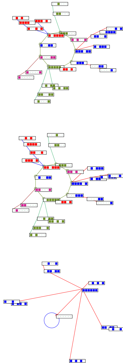
Figure 31.21: If transient data was set in 31.7 ( include trans data=t ) it will be included with attractor data in section 31.7.6. This example is for a very small CA v2k3 (elementary rule) n=6 rcode 110. The basins of attraction with nodes as bits are inset on the right for comparison (see also figure 24.2). In this case the sample has revealed all attractor states, and all transient states — without duplication. The same type of data can be listed for larger networks, or for RBN and DDN.
