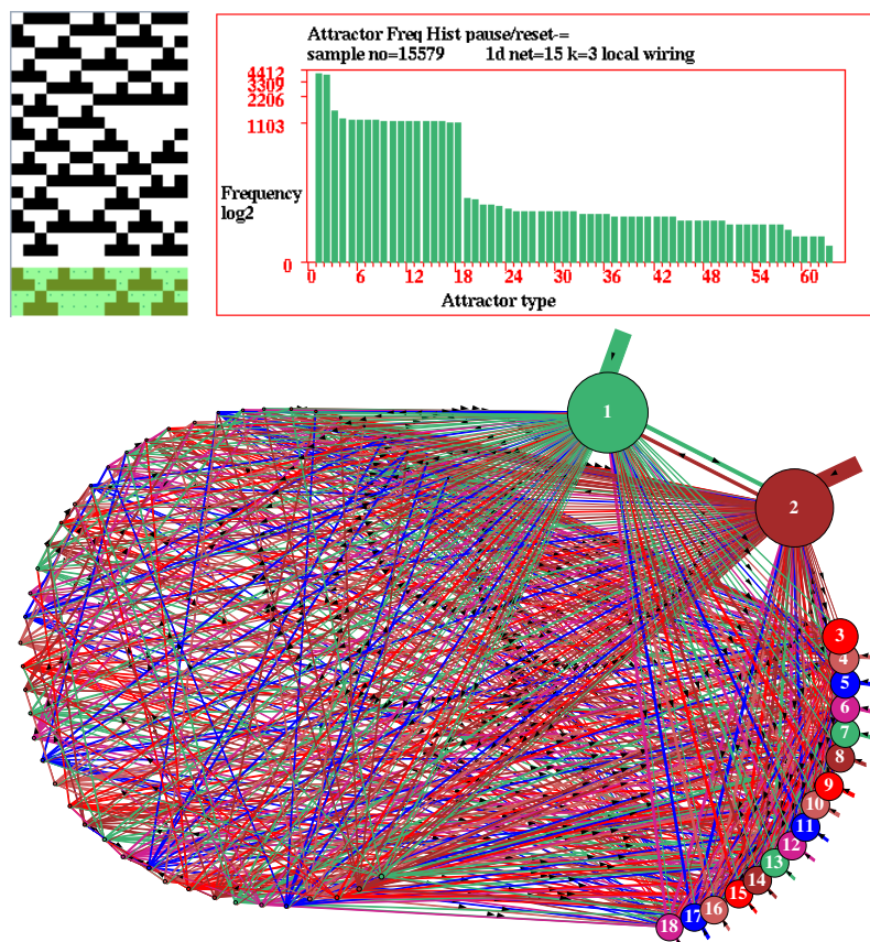
Figure 31.22: The attractor histogram jump-graph, for a 1d CA, v2k3 rcode(dec)54, n=15 . Top left: a sample space-time pattern showing the attractor repeated. Top Right: The attractor histogram with log y -axis, all 63 attractors were found after a sample of 15579. Above: the h-jump-graph (section 20.7) — nodes scaled by basin volume and links jump probability, and the graph rearranged (section 20.10) starting from a circle layout.
