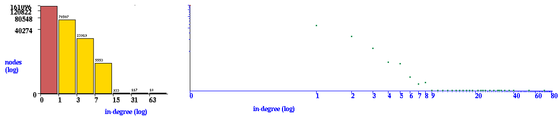
Figure 24.7: The in-degree histogram as a log-log plot can be implemented in two ways on the x -axis, Left : preserving a histogram (the default) with bins that capture an increasing range of in-degrees, 0, 1–2, 3–7, 8–15, etc. Right : a simple log-log plot. The x and y axis can also be treated separately. These plots are for the CA, v2k3 rcode (dec)193 , in figure 24.6.
