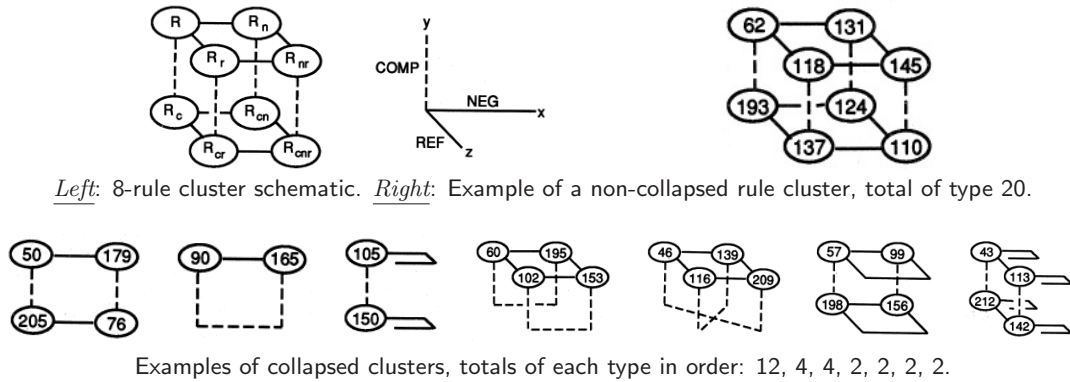
Figure 22.4: Graphical representation of rule clusters of the v2k3 “elementary” rules, and examples, taken from “The Global Dynamics of Cellular Automata” [38] section 3.3, where it is shown that the 256 rule-space breaks down into 88 equivalence classes and 48 clusters. The rule cluster is depicted as 2 complementary sets of 4 equivalent rules at the corners of a box — with negative, reflection, and complementary links on the x, y, z edges, but the edges also collapse due to symmetries.
