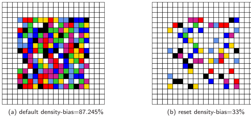
Figure 21.5: Setting the v=8 density-bias for a central block 14 \times 14 within a 2d seed i, j=20 \times 20 , showing the default and reset density. The graphic output would appear as in figure 21.4, but is presented here from “Setting the seed as bits or values” (section 21.4).
