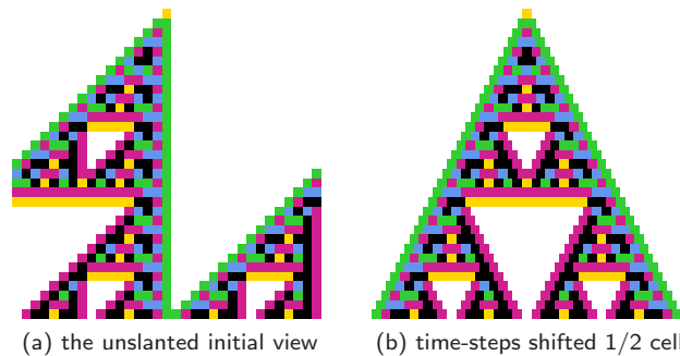
Figure 16.15: 1d v8k2 periodic space-time pattern of an isotropic CA, size 33, showing 33 timesteps from a singleton seed. The rcode size=64, The iso-rule (size=36): 140761540026777563655513706072505220, as a graphic: and in hexadecimal: 07 07 c6 c0 16 ff dc f5 b4 be 30 ea 8a 90. (a) is the initial view because 1d even n -templates are skewed right (figure 10.1). (b) central symmetry restored with on-the-fly "slant" option (section 32.9.1), which shifts successive time-steps by 1/2 cell — so k in 1d CA can be even as well as odd with a valid iso-rule.
