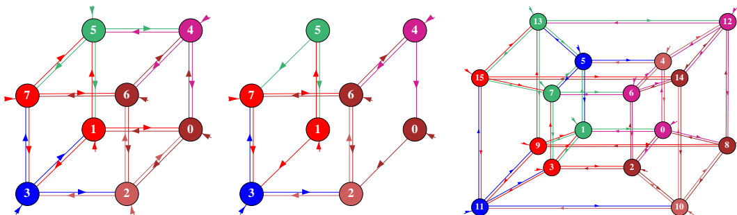
Figure 12.1: Hypercube wiring shown as a network-graph (section 20.5). Left : n=8 k=4 hypercube, which includes self-links. Center : a degraded version of the n=8 hypercube with some links missing. Right : n=16 k=5 hypercube. The 3d-3 network-graph option was used for the figures, and the graph was rearranged by dragging nodes (section 20.10). The figures should be viewed as if looking up from below. Output directed links are the same color as the source node. To regenerate these layouts automatically, enter file-f in section 20.7.3 for the filing prompt (section 35.3) and load the *.grh layout file, hyp8 or hyp16 (.grh is added automatically).
