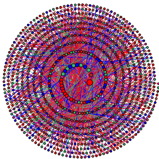
Figure 20.17: Ranked spiral layout of the ibaf-graph in figure 20.22 with 2^{10}=1024 nodes. Starting at the center, nodes are ranked by descending node size based on in-degree — garden-of-Eden states with in-degree zero form the outer layers. Equal sizes are in descending order of the state’s decimal value (1d CA v2k3 , n=10 , rule 110).
