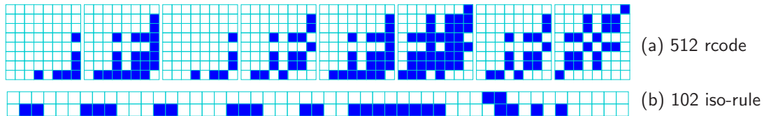
Figure 16.4: (a) the 512 bit rcode graphic of Conway's game-of-Life ( s23/b3 ) shown in 8 rows. The diagonal symmetry in each 8 \times 8 block is a necessary (but insufficient) indication of isotropy but a useful visual clue for the general case of isotropic rcode for a binary v2k9 2d CA with a Moore neighborhood. (b) the 102 bit iso-rule, transformed from rcode with R (from options >iso-I/R/H/* ).
