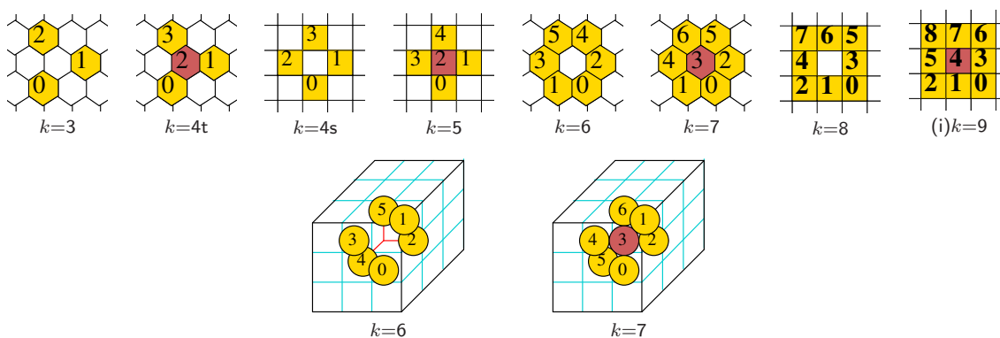
Figure 16.17: Predefined neighborhood templates valid for iso-rules: any 1d n-template is valid, and also those shown above for 2D ( k=3 to 9) and 3d ( k=6 or 7). 2d k=4 n-templates can be either hexagonal or square. To achieve periodic boundary conditions hexagonal n-templates require even lattice dimensions. The target cell is central even if not part of the n-template.
