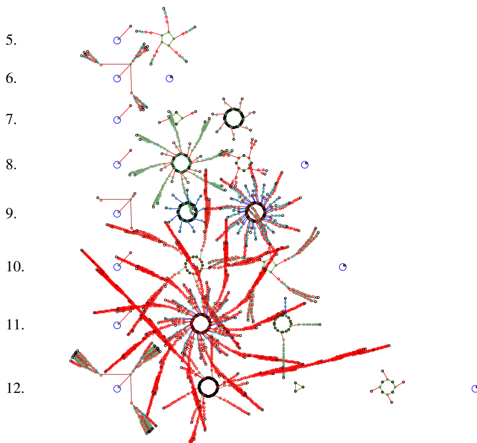
Figure 4.6: Basin of attraction fields for a range of network size n=5-12 . v2k3 , rule(dec)=30
