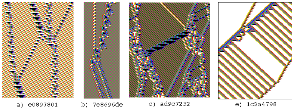
Figure 32.6: Examples of 1d v2k5 complex space-time patterns with interacting gliders[39] from a GRC file ( g_v2k5.r_s , section 3.6.1) included with DDLab, which can be loaded on-the-fly while space-time patterns are being drawn (cells colored by neighborhood, section 31.2.1). The rcodes are shown in hex.
