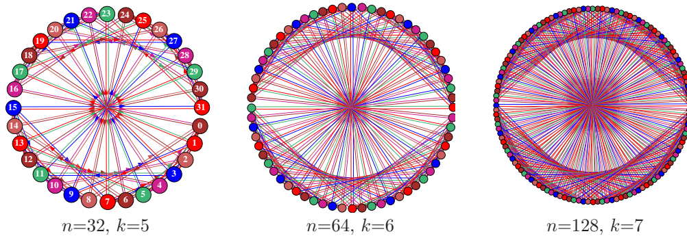
Figure 12.2: Hypercubes for n \geq 32 are difficult to visualise in 3d. These examples show hypercubes as a network-graph with circle layout (section 20.5).
