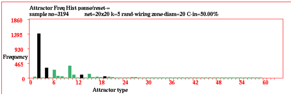
unsorted histogram, for a sample of 3194
