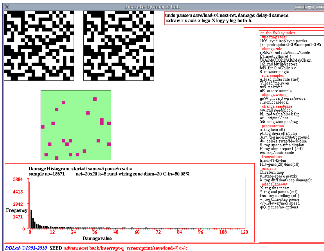
Figure 31.15: The DDLab screen, showing the automatic process for gathering statistics on (actual) damage. This example is for two 20 \times 20 RBN, k=5 , with canalyzing inputs set to 50%, (chapter 15). At each pass, a new random initial state is assigned to the sub-networks, differing by one bit at a random position. When the damage stops spreading, the histogram of the damage size ( x axis) against the frequency of damage size ( y axis), is updated. The process was paused with the = key.
