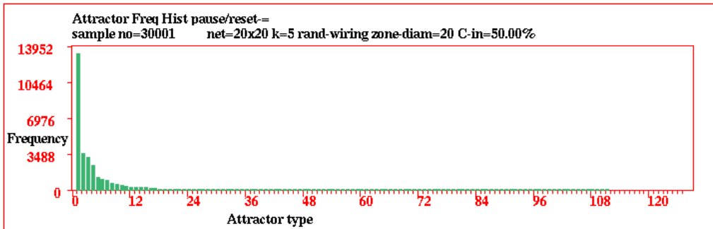
sorted histogram, according to frequency, for a sample of 30001, with 111 attractors
