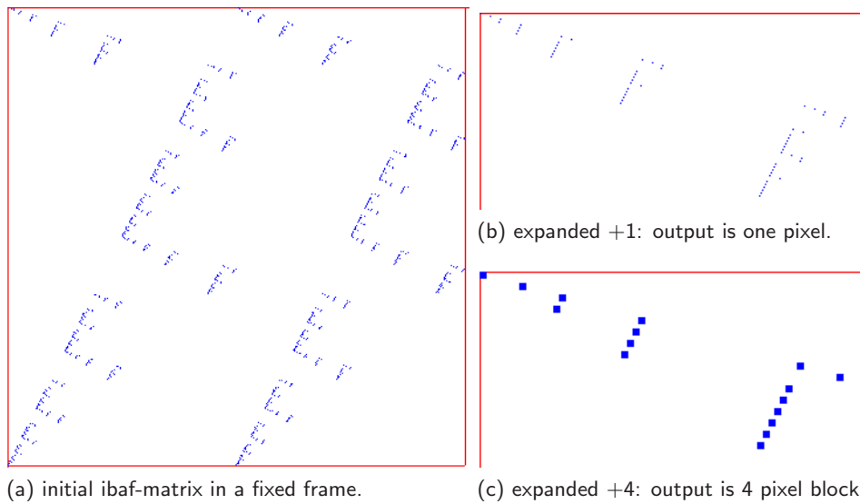
Figure 20.25: The ibaf-matrix of the ibaf-graph for the v2k3 CA rcode 30 n=10 with E=v^n=1024 states in 6 basins (ibaf-graph figure 20.26). Compare the pixel-pattern with the return map for the same rule (figure 31.5). (a) The initial E \times E matrix is confined within a fixed size frame. The matrix can be expanded, showing as much as will fit. (b) The expanded matrix, still with single pixels — top left area. (c) Expanded to 4-pixel blocks — top left area.
