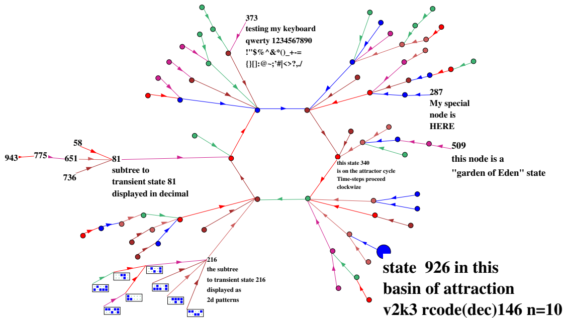
Figure 20.19: An example of arbitrary labels in the ibaf-graph with “ Label-L ” — the methods apply equally to the network-graph and jump-graph. In this example the ibaf-graph has unscaled nodes and edges, and the basin was isolated with “ just-j ”. The default label start position is just below current state display which can still be toggled (key ‘=’) for single states or fragments — for example the subtree to state 81 has been toggled to show all its inputs as decimal numbers, and the subtree to state 216 as 2d patterns.
