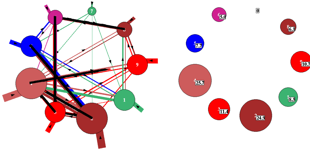
(a) The ant has a red body and leaves a black trail. (b) The percentage of ant hits at each node after 5 million moves — with ant animation disabled this took a few seconds. Node 7 indicated by 7 is unreachable from other nodes so has zero hits.
