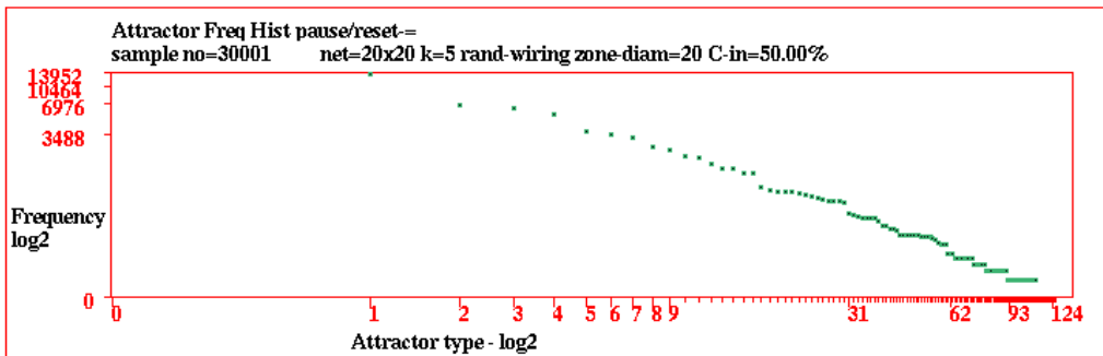
The sorted histogram, shown as a log-log plot
