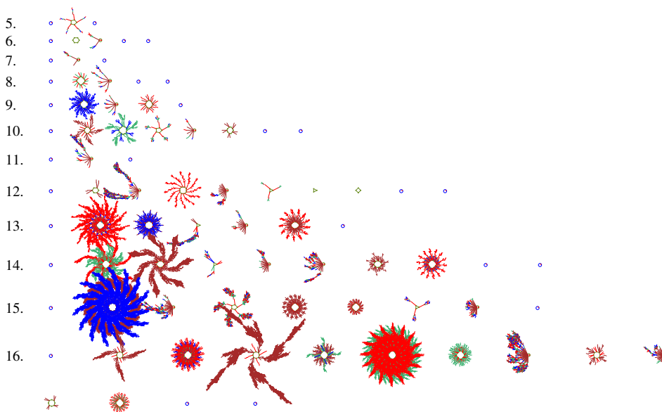
Figure 25.5: The basin of attraction field for a range of network size, n=5-16 , shown on the left, v2k4 rcode (hex)8b26. The spacing between basins increases at a set rate as larger basins are expected for greater n . In this example, the basin scale is 1.2 (section 25.2.4), the x, y start position is -90,70 (section 25.2.5), the initial x, y spacing between basins is 6,6 (section 25.2.7), the right border width is 45% (section 25.2.8), and the x, y spacing increase is set at 12%.
