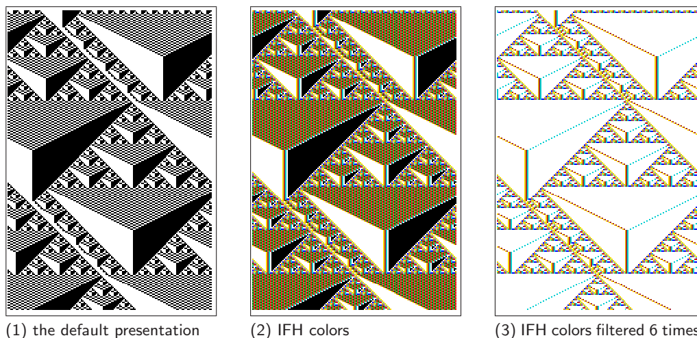
Figure 32.32: Tap : (a)-(f) adjusting IFH bar length with 32 bars of the 1d v2k5 rcode, and filtered 6 times with keyhit 'f' (section 32.11.5). Above : (1)-(3) alternative presentations of the same 1d STP, size n=150 , 223 time-steps, from the same initial state. The rule is Wentian Li's[28] v2k5 rcode (hex)c3bce390 (complex collection 33) also shown in figure 32.31.
