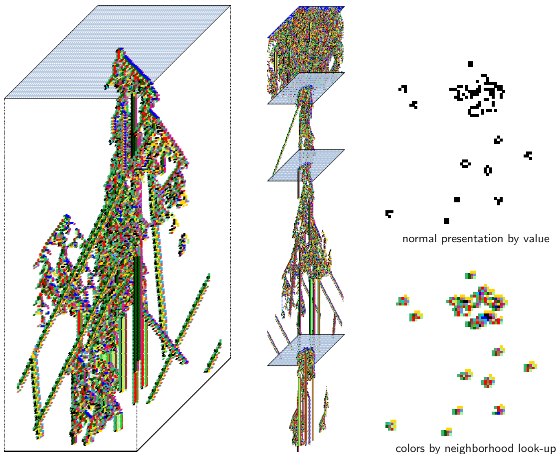
Figure 4.12: Space-time patterns of the 2d game-of-Life, ( k=9 , n=66 \times 66 ) with time-steps stacked below each other in a isometric projection scrolling upwards. Left: starting from the “r-pentomino” seed. Center: re-scaled to the smallest scale, with new seeds set on-the-fly at intervals. Upper Right: The state at time-step 230. Lower Right: the same state colored according to the neighborhood look-up instead of the value.
